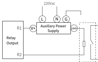
Relay output
