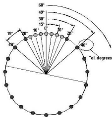
Figure 2: Physical and electrical position of LEDs
