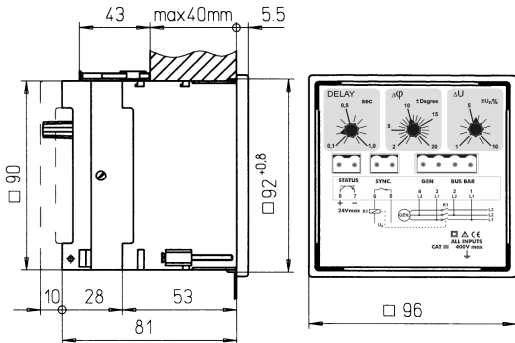
Figure 5: External dimensions in mm
