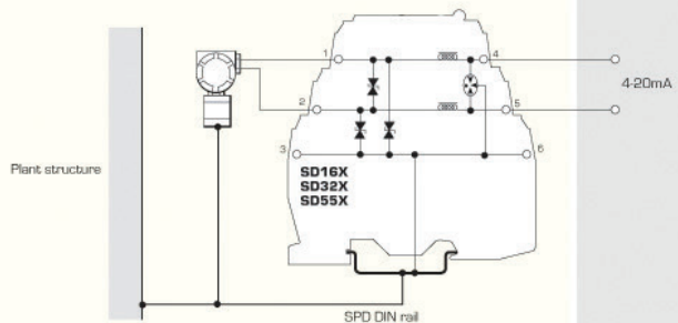
2-wire transmitter or sensor
