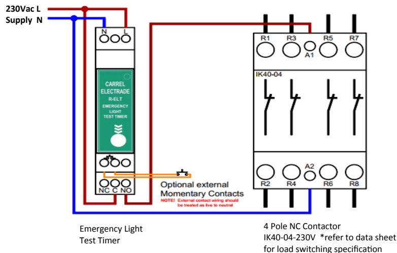
R-ELT + NC CONTACTOR CONNECTION DIAGRAM
